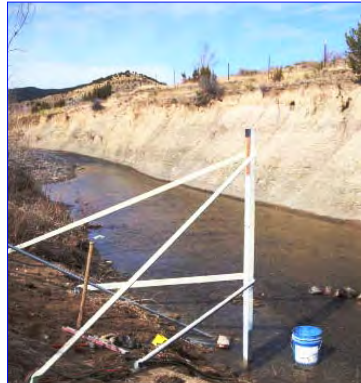
Bubbler & Orifice Line
